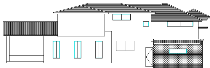
1. PROPOSED SOUTHERN ELEVATION
